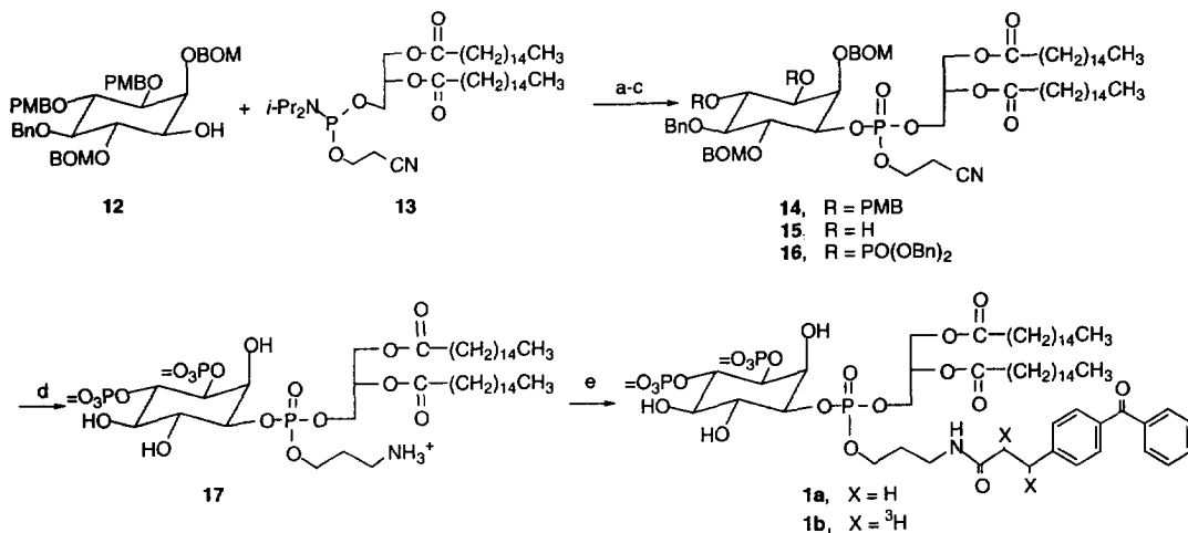
Scheme 2. Coupling and conversion to affinity probe. Reagents and conditions: (a) (i) 1 H -tetrazole, CH 2 Cl 2 , rt, 1 h; (ii) m -CPBA, CH 2 Cl 2 , -40 °C to rt, 30 min; (b) DDQ, wet CH 2 Cl 2 , rt, 5 h; (c) (i) 1 H -tetrazole, (BnO) 2 PN( i -Pr) 2 , CH 2 Cl 2 , rt, 1 h; (ii) m -CPBA, CH 2 Cl 2 , -40 °C to rt, 1 h; (d) H 2 , Pd/C (10%), NaHCO 3 , t -BuOH/water, 22 h; (e) BZDC-NHS, 0.25 M TEAB, DMF, rt, 18 h. The symbol "=" in the phosphates denotes the presence of a counterion (H + , Na + , Et 3 N + ) appropriate to each solution or stage of purification.
